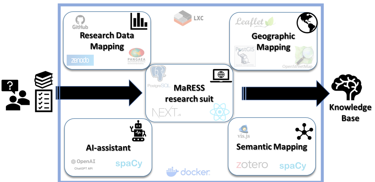
Figure 1: Modular design of the MaRESS research suite, integrating four key modules—Research Data Mapping, Geographic Mapping, Semantic Mapping, and AI-Assistant. Each module addresses distinct aspects of data management and analysis in Earth System Sciences (ESS) to build a comprehensive knowledge base from initial user input. Semitransparent annotations indicate selected open-source tools, libraries, and open-access platforms integrated into or connected with MaRESS.
